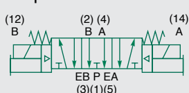
double solenoid 3 Position 4-Way (5/3), open to 4 (A) and 2 (B) in center
