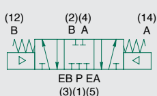
double solenoid pilot 2 position 4-way
