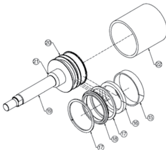
Piston/Rod Assembly
