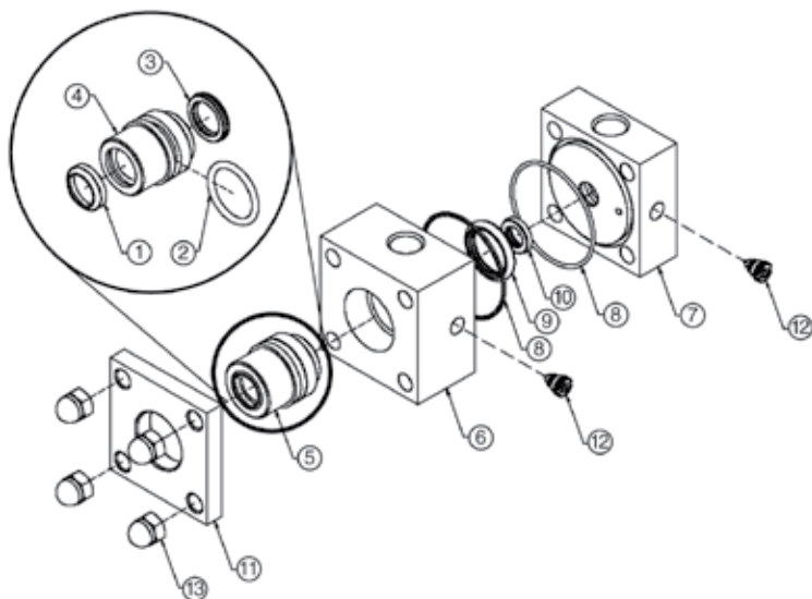
Head, Cap, and Bushing Assembly
