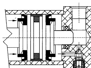
Silencer Bumper Seal EB option
