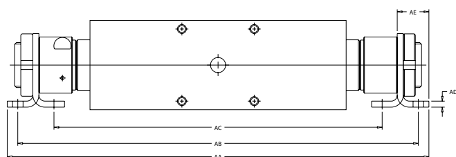
MC1 & MC2 - 32 MM AND 40 MM BORE FOOT MOUNT
