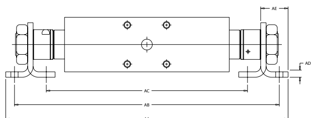
MC1 & MC2 - 32 MM AND 40 MM BORE FOOT MOUNT
